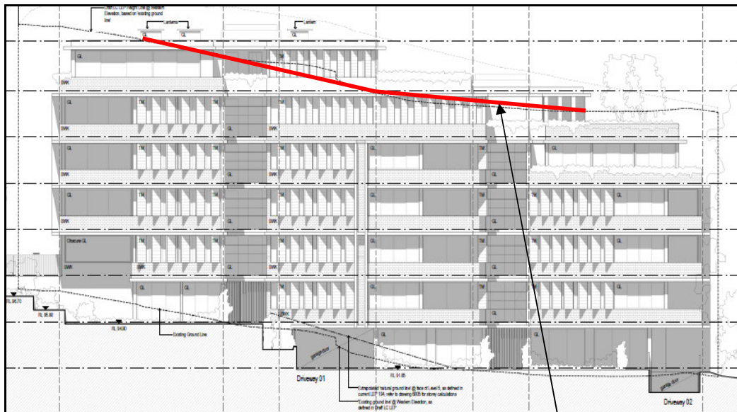
Figure 5 – Western elevation
